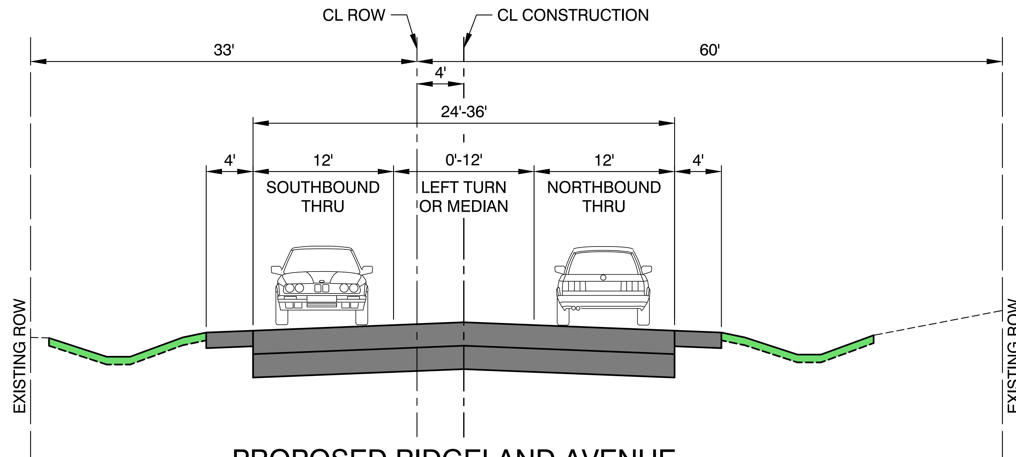
PROPOSED RIDGELAND AVENUE SOUTH OF 175TH STREET
