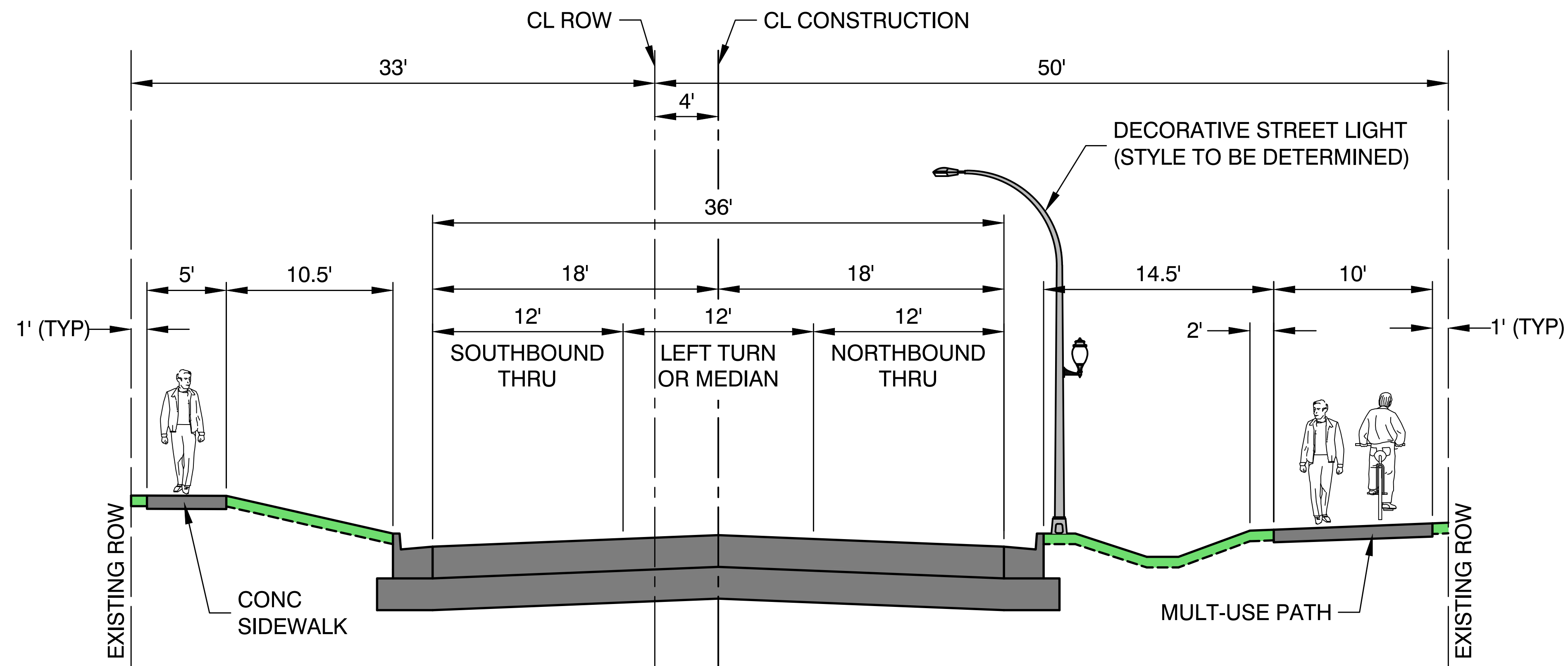
PROPOSED RIDGELAND AVENUE 175TH STREET TO OAK FOREST AVENUE
